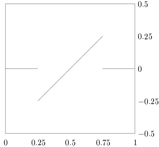
Figure 11: Haar series partial sum S_{256} , which has 257 terms.
